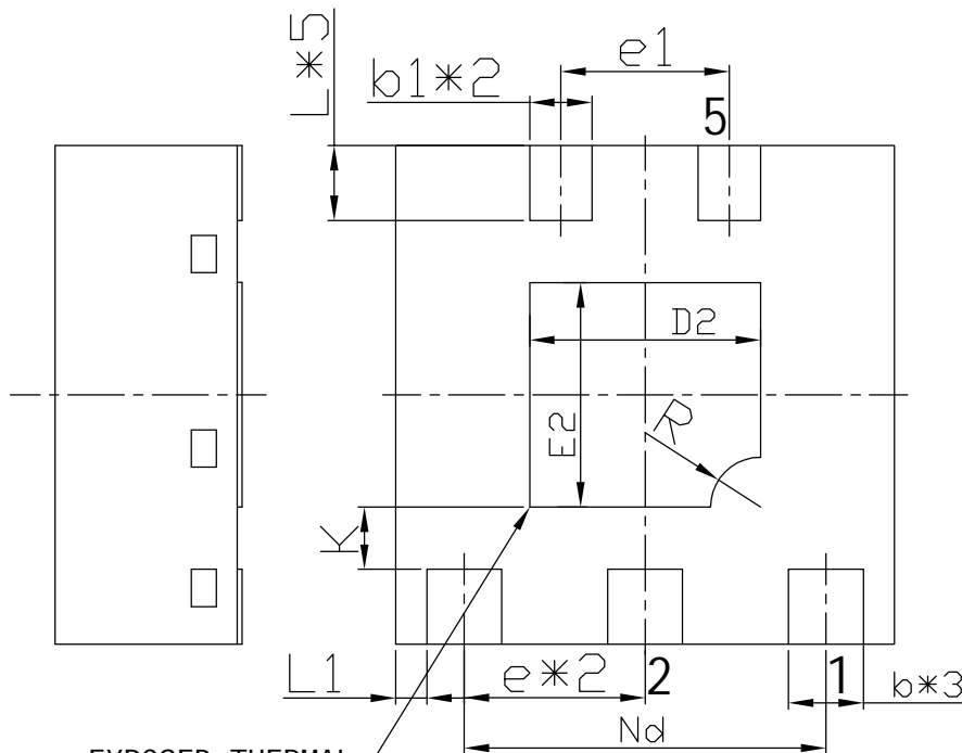
BOTTOM VIEW
