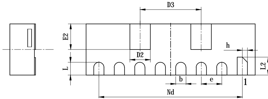
BOTTOM VIEW
