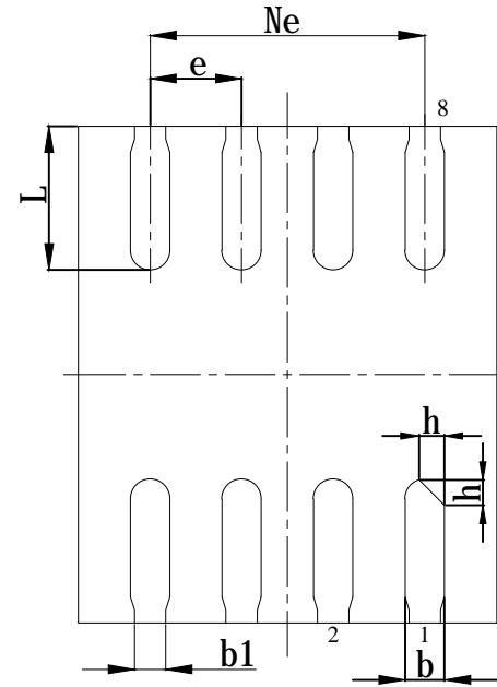
BOTTOM VIEW
