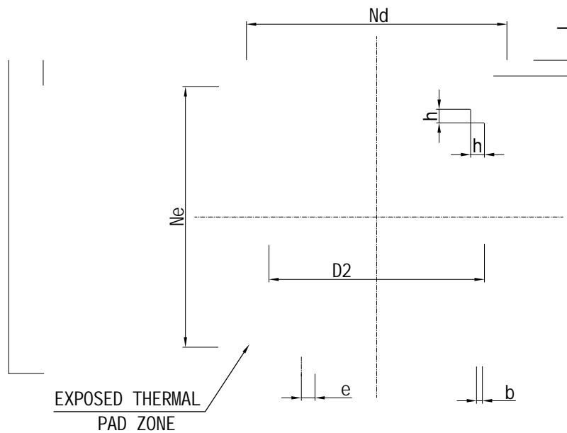
BOTTOM VIEW
