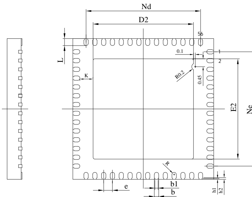
BOTTOM VIEW
