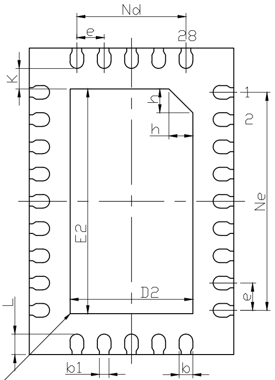
BOTTOM VIEW
