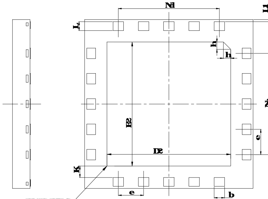
EXPOSED THERMAL PAD ZONE
